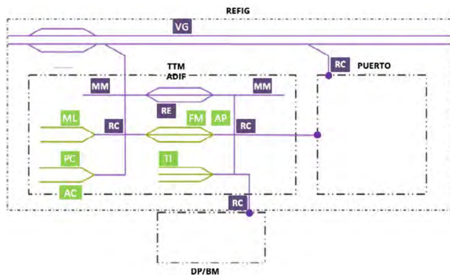
Figure 1. Functional Schematic of an Adif Freight Transport Terminal (T.M. ADIF).
