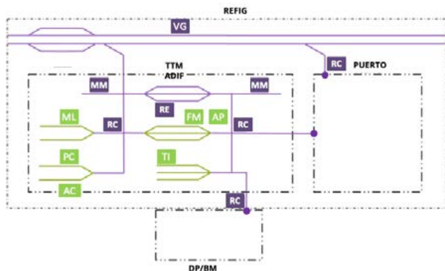
Figure 1. Functional Schematic of an Adif Freight Transport Terminal (TMM ADIF).
